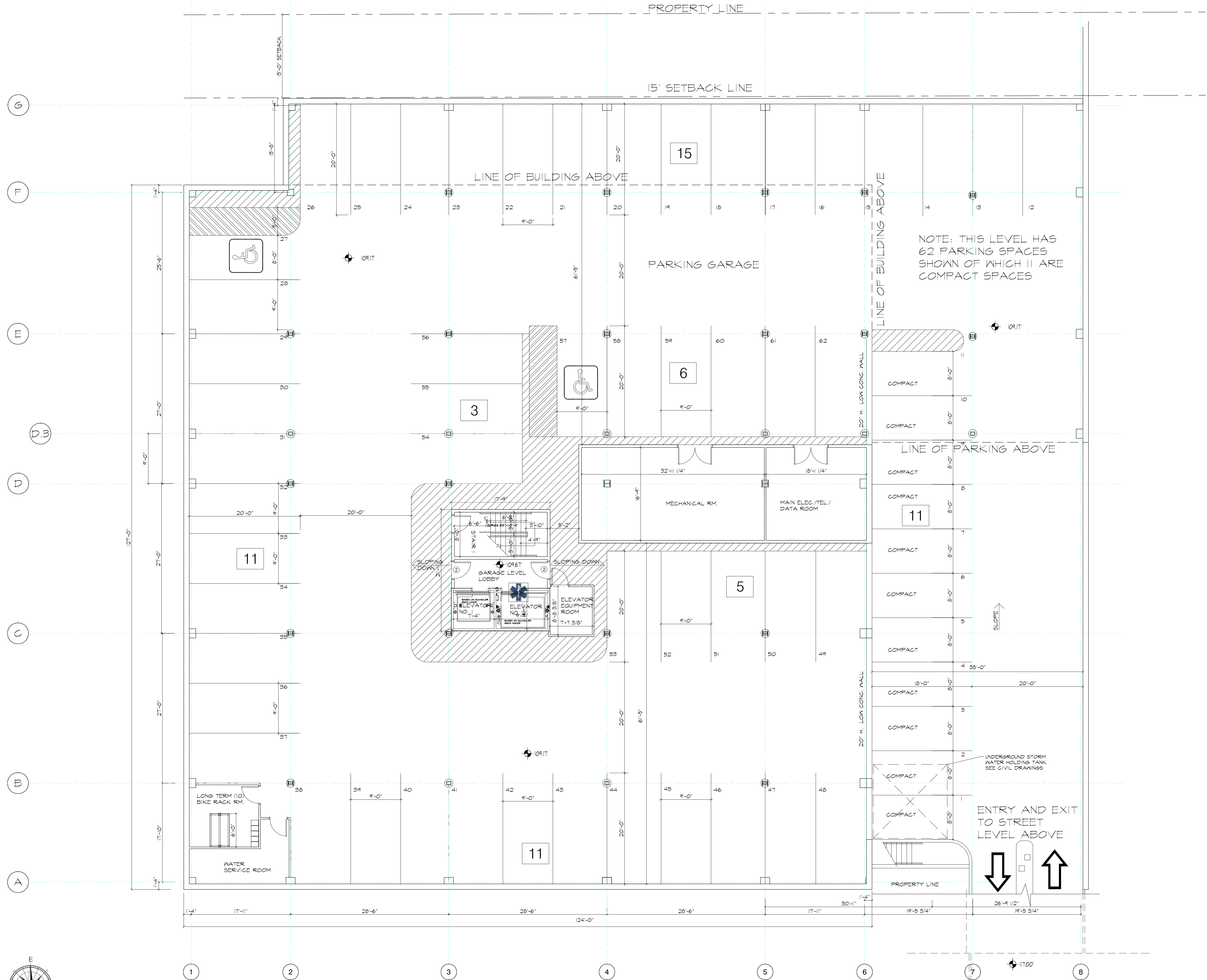
GARAGE FLOOR PLAN SCALE: 1/8" = 1'-0"
