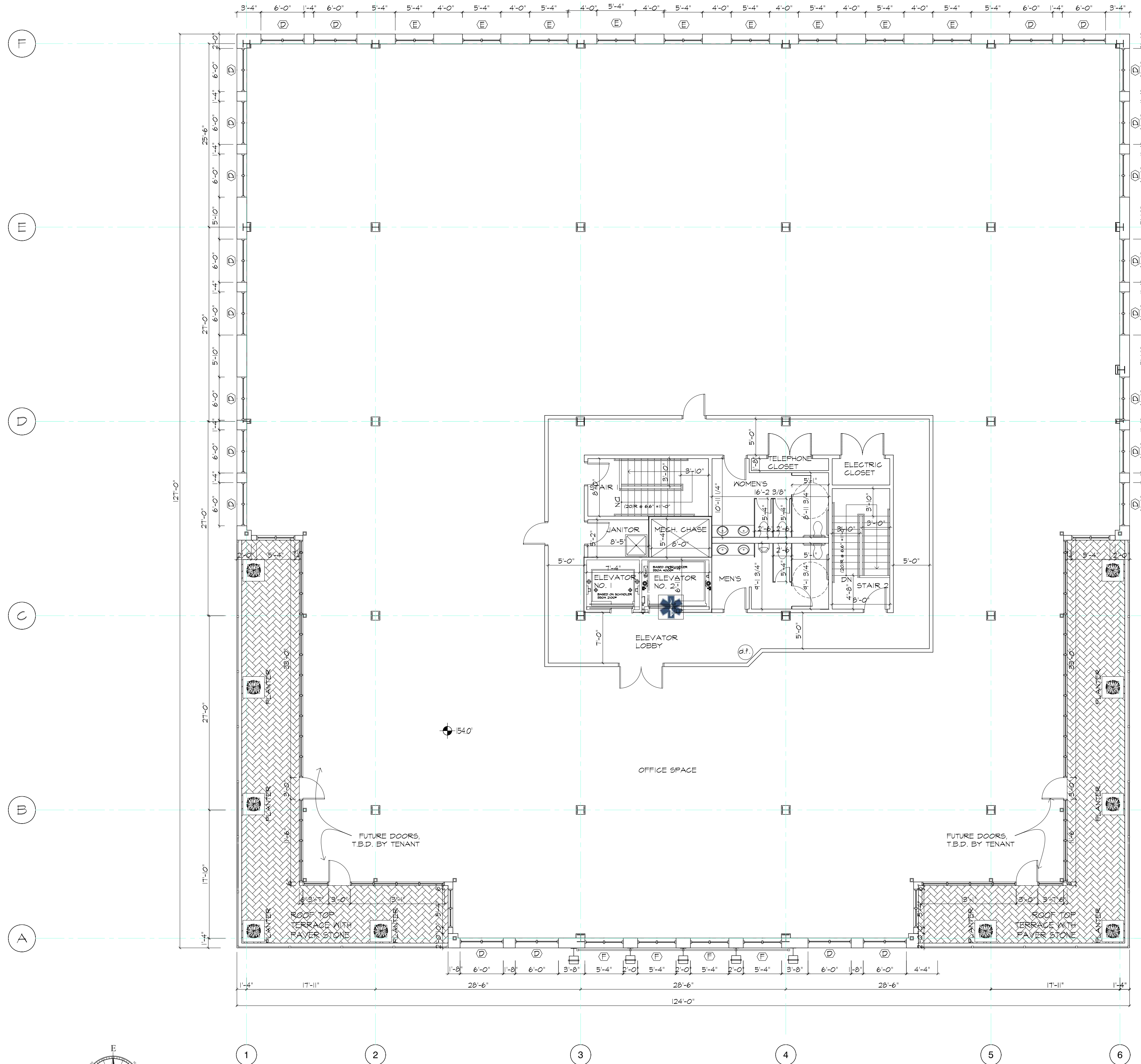
4 4th FLOOR PLAN SCALE: 1/8" = 1'-0"
